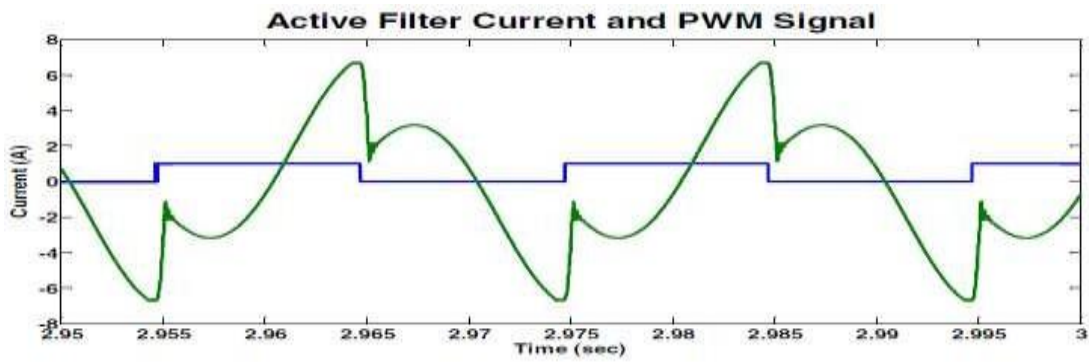
Fig. 6: Active filter current and PWM signal
