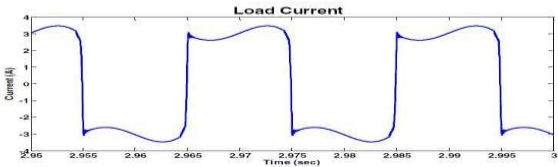
Fig. 7: Load current
