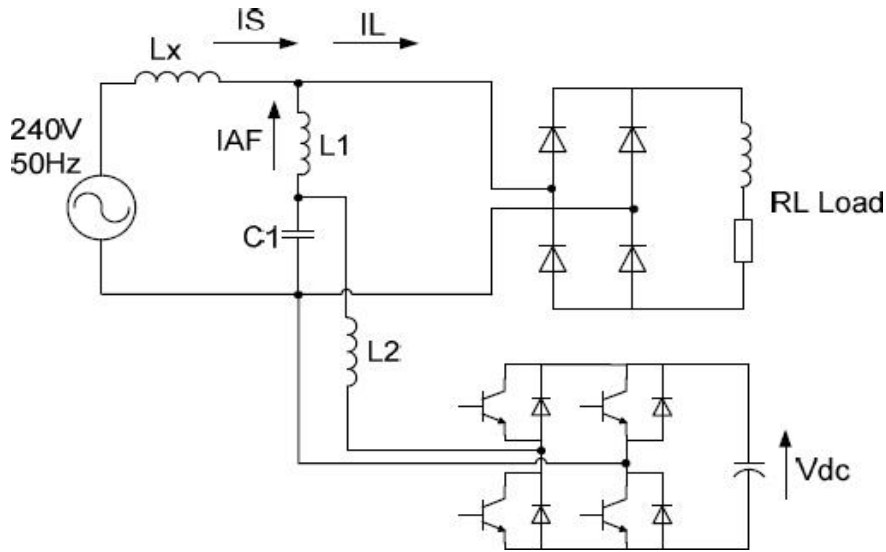
Fig. 1: Schematic diagram of single phase shunt active filter
