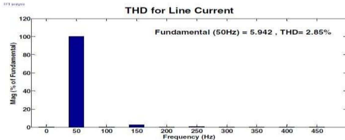
Fig. 10: THD for line current
