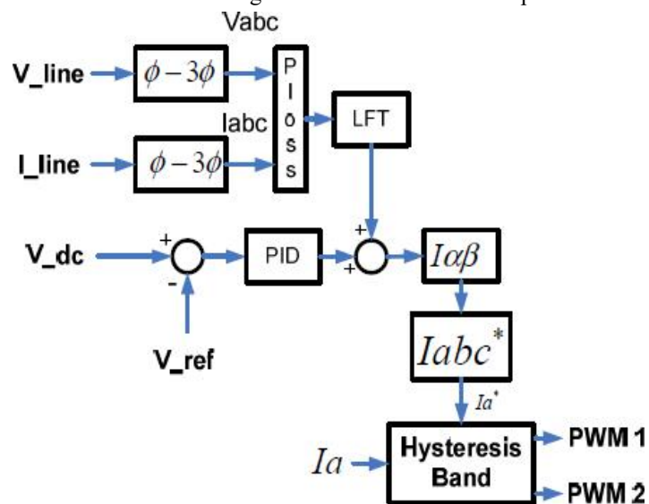
Fig. 2: Control strategy
