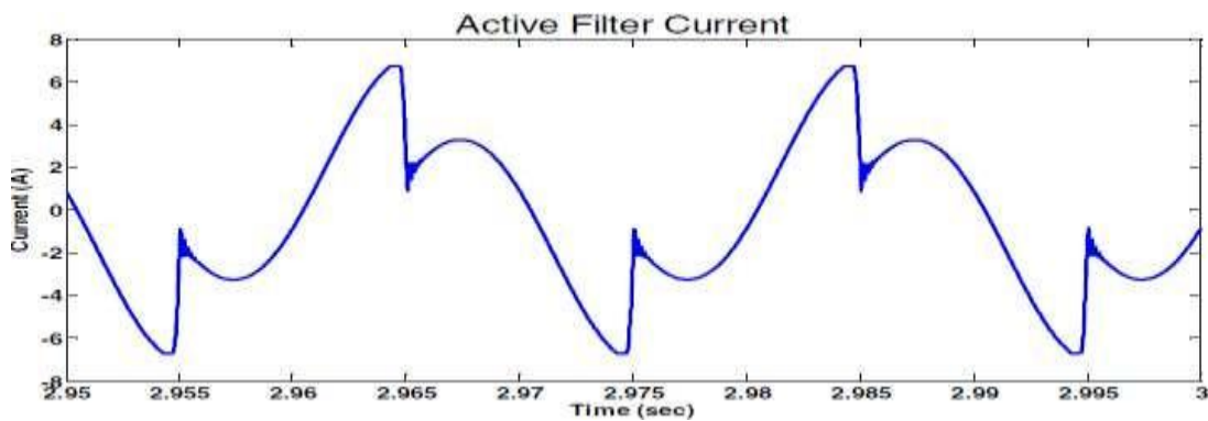
Fig. 8: Active filter current
