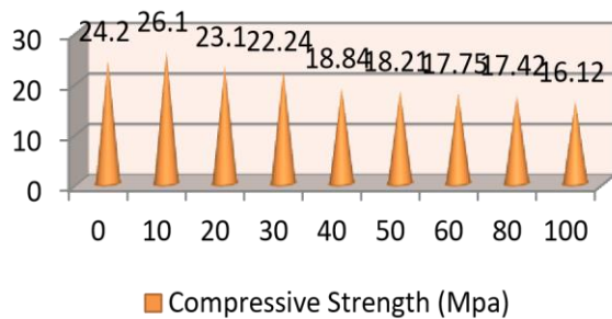
Fig. 4. Variation in Compressive Strength cured for 28 days for various percentages of RA.
