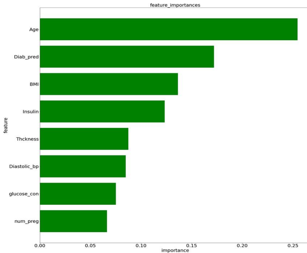
Feature3: Importance for Diabetes Dataset
