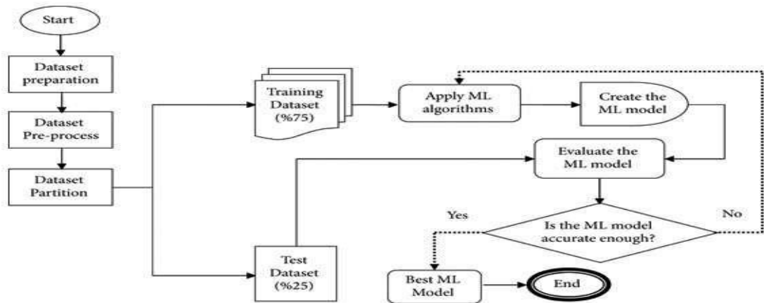
Figure 1: Sequences of the proposed approach for predicting diabetes.
