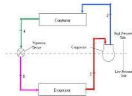
Fig-1: Schematic diagram of simple VCRs Fig-2: Actual Setup of LPG Refrigerator Fig-3: Actual Setup of LPG Refrigerator
