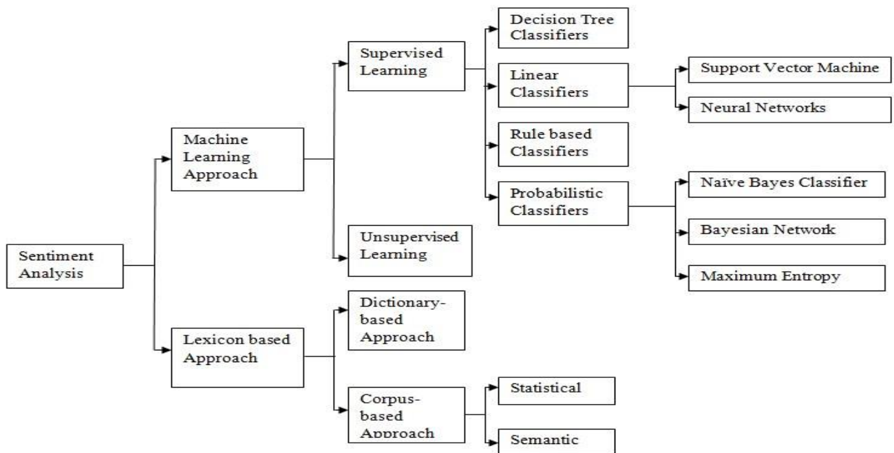
Fig 2: Sentiment Analysis Techniques
