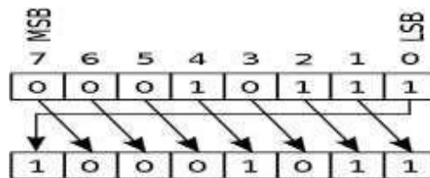
Fig3.2 Right circular shift operation Steps are for implementing the booth algorithm:
