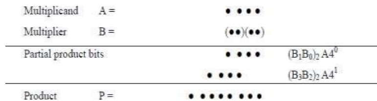
Fig3.8 Radix-4 multiplication in dot notation
