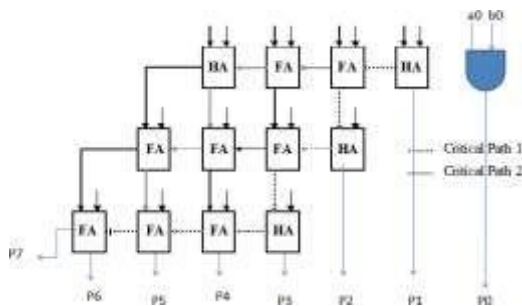
Fig3.1 Architecture of array multiplier boao is generated by using AND gate
