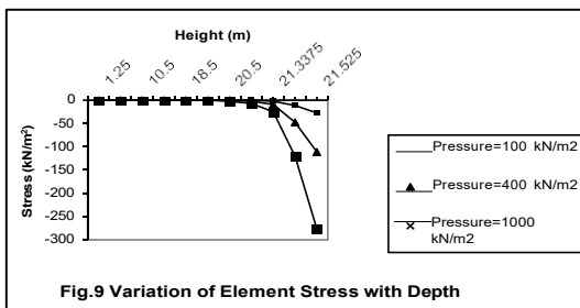
Fig.9 Variation of Element Stress with Depth
