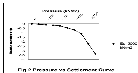
Fig.2 Pressure vs Settlement Curve
