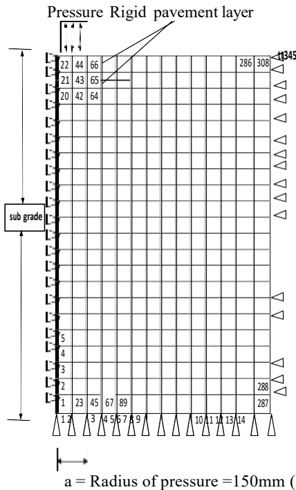
a = Radius of pressure =150mm (Fig not scale) Fig.1(a). Finite Element Discretization for Rigid Pavement without Base course
