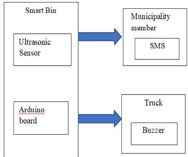
Fig.3. Block Diagram
