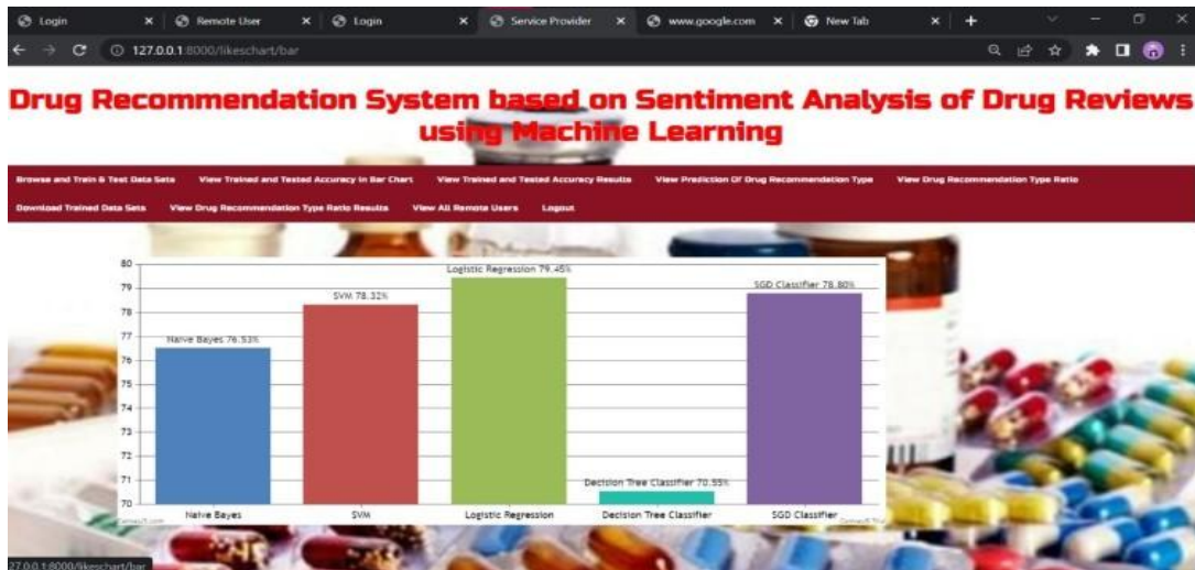
Figure4 : Chart showing Accuracy using various ML Models
