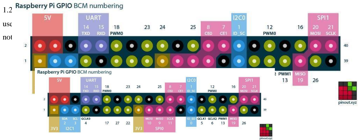
Figure 2: illustration of Raspberry pi 3B GPIO's
